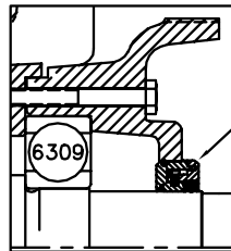
PULLEY END DETAIL
