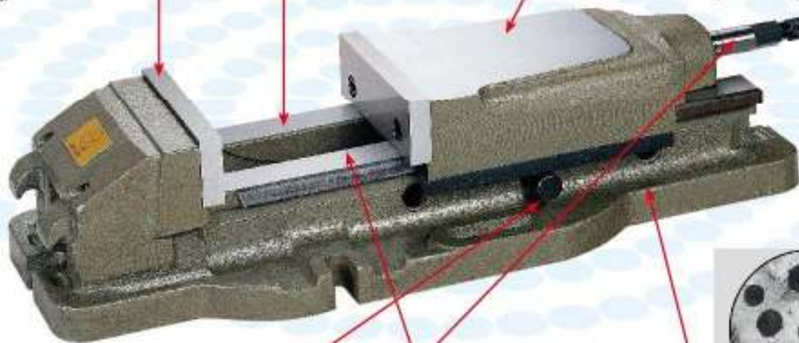
Patented new device hydraulic cylinder
