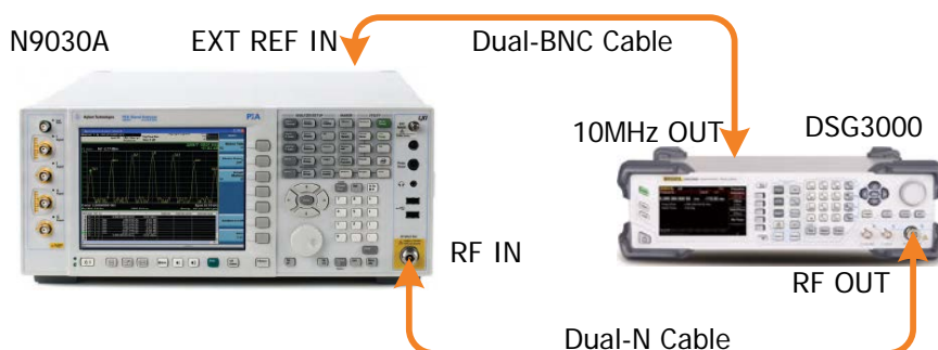
Figure 2-4 Second Harmonic Distortion Test Connection Diagram
