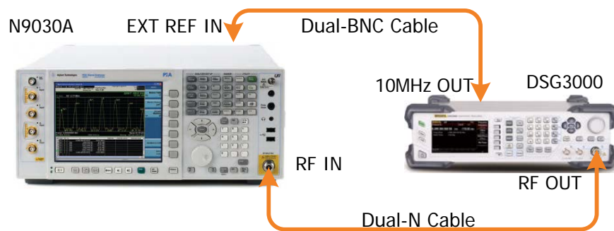
Figure 2-2 Single-sideband Phase Noise Test Connection Diagram
