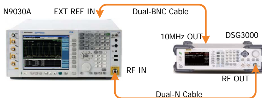
Figure 2-6 FM Internal Modulation Test Connection Diagram
