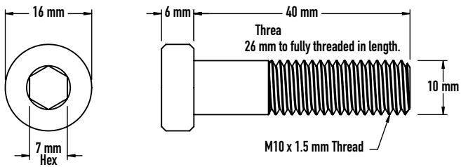
2x Low Profile M10 Socket Head Cap Screw
