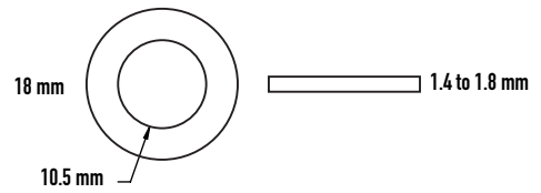
2x M10 Washer
