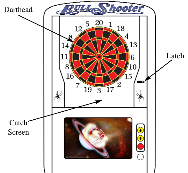
15" Darthead Face
