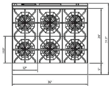
6 Burner Range top view
