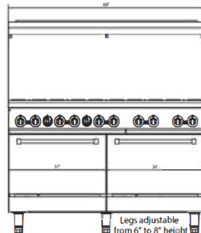
10 Burner Range front view
