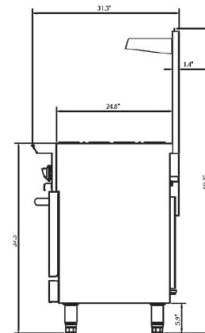
10 Burner Range side view
