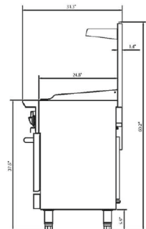
Griddle Range side view
