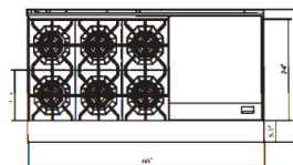
Griddle Range top view
