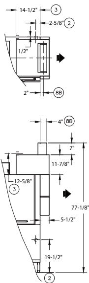
Model RCT 64 or RCT 84 Roller Conveyor Table
