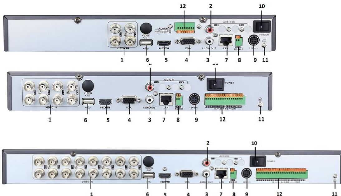
Figure 1. 5 Rear Panel of 4/8/16ch 720p Series with alarm
