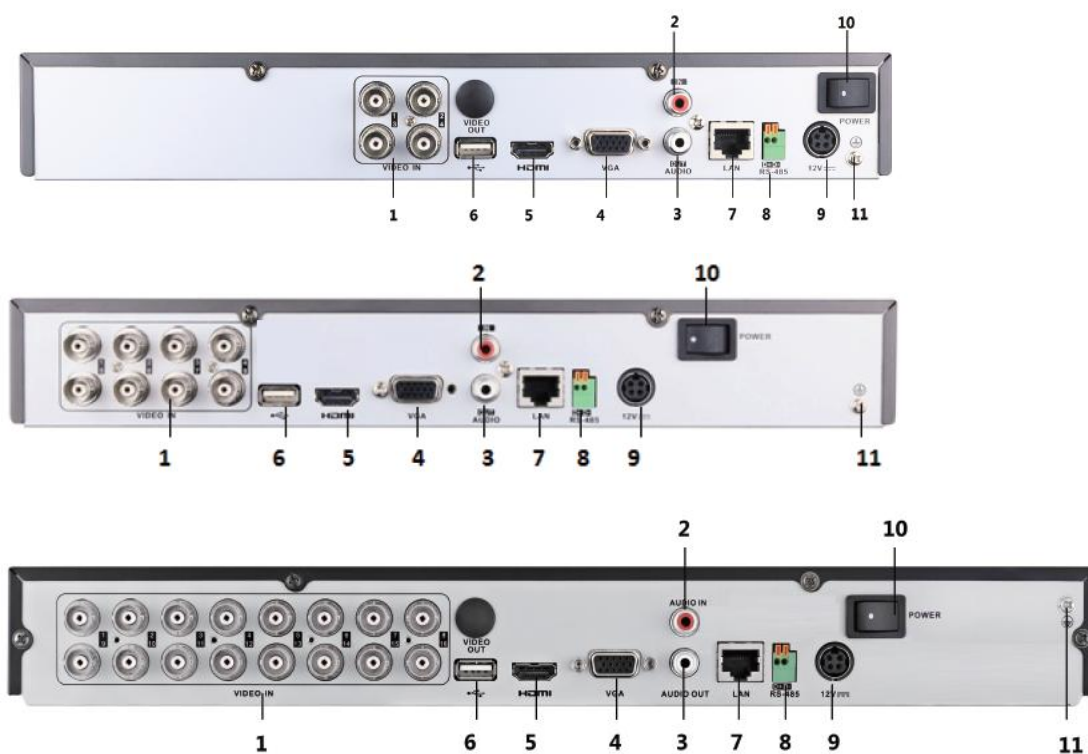
Figure 1. 4 Rear Panel of 4/8/16ch 720p Series without alarm
