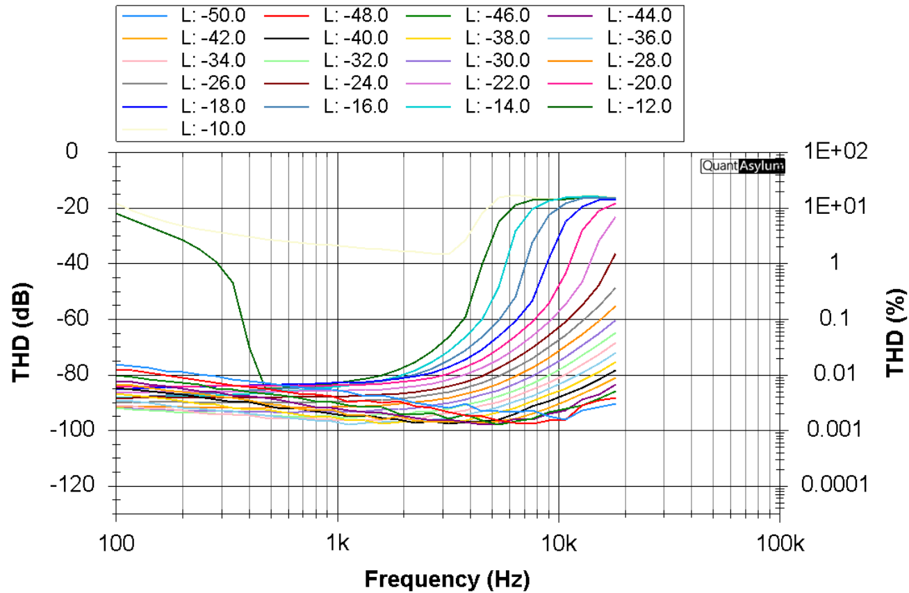
QA472 PRE2 THD versus Frequency and Amplitude
