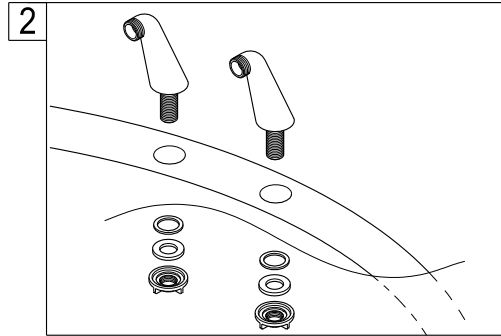
2. Place risers on the tub, tighten the lock nuts from underneath and connect the water supply lines. Place washers and tighten the coupling nuts on to the mounting legs.
