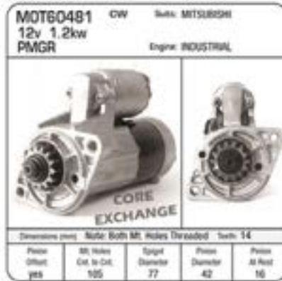
MOT60481 STARTER 12V MITSU IND 14TH Manufacturer: Mitsubishi
