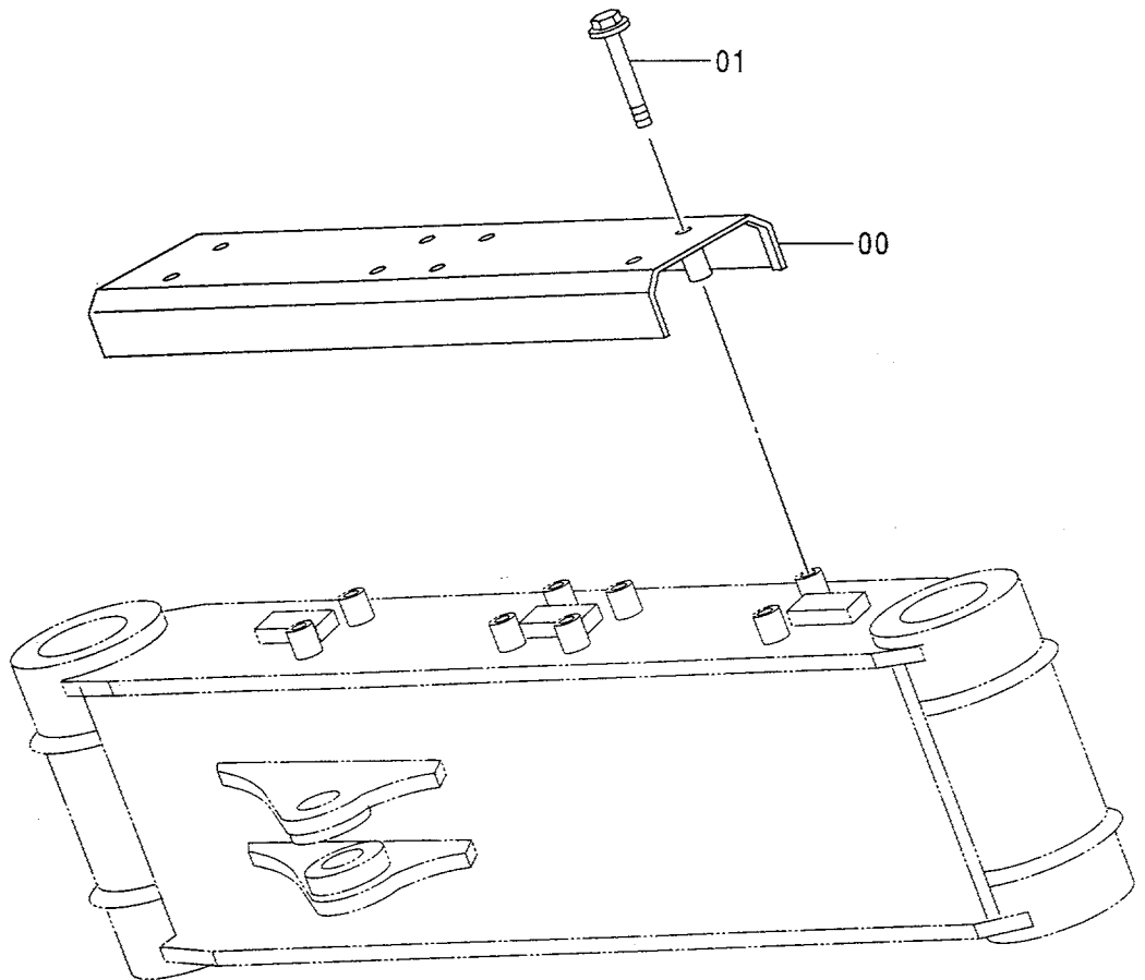
側溝掘boom OFFSET BOOM
