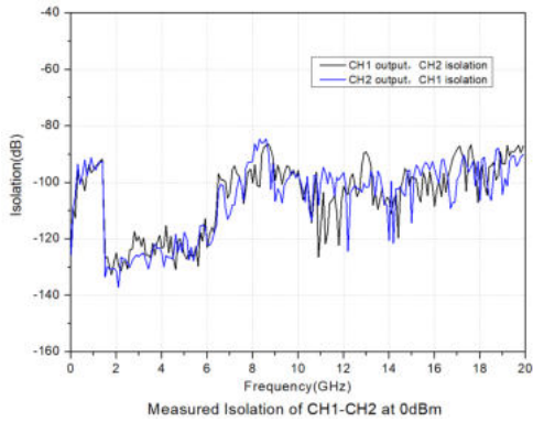
Channel-to-channel isolation
