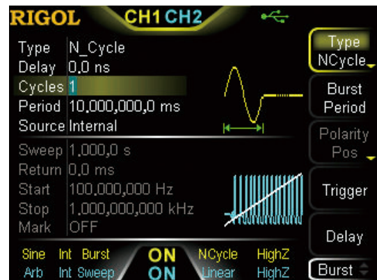
Burst function
