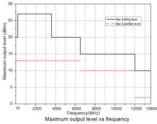
Maximum output level vs frequency
