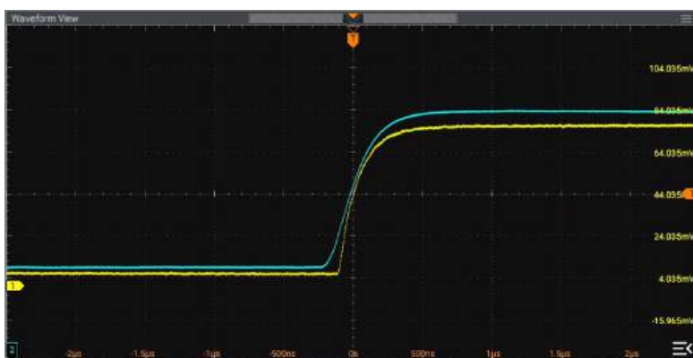
Channel Deskew
