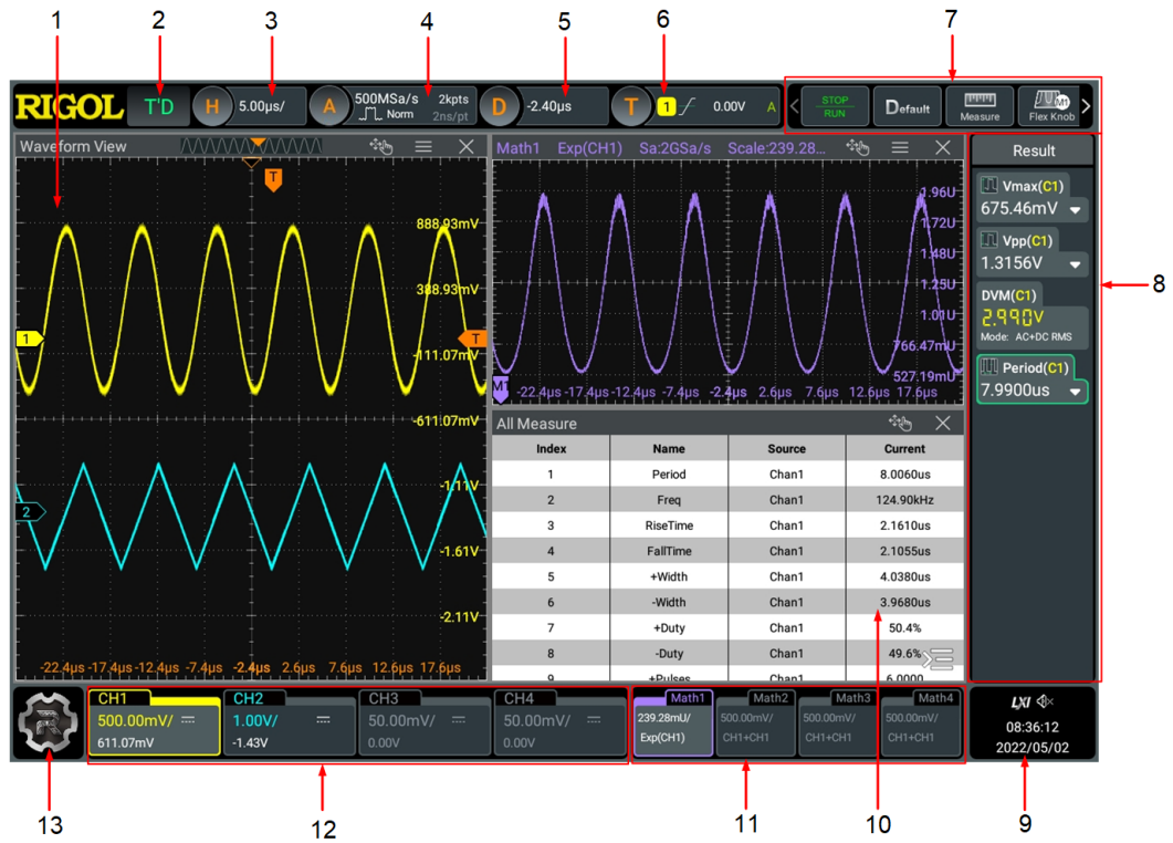
Figure 4.4 User Interface
