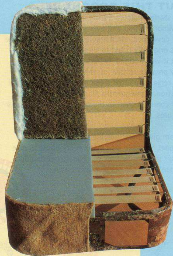
Typical seat make up of the internal items required for cars from 1956- 1971
