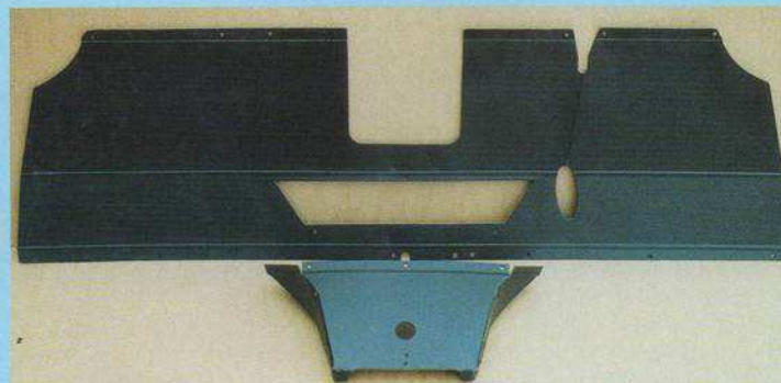
Mid range parcel shelf with the duct to cover the front of the heater unit
