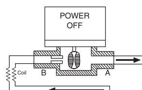
Figure-6b 2-Way Valve With Normally Open Actuator
