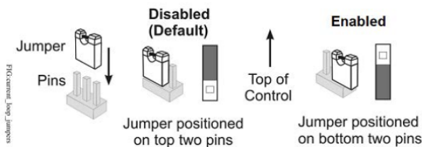
Figure 9: Current loop jumper positions
