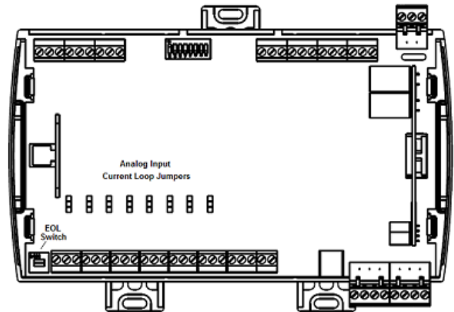
Figure 8: Cover removed showing EOL switch and jumper positions
