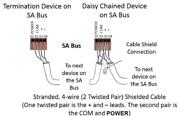
Figure 4: SA bus terminal block wiring
