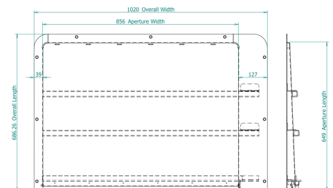
PSV Manual Ramp Narrow
