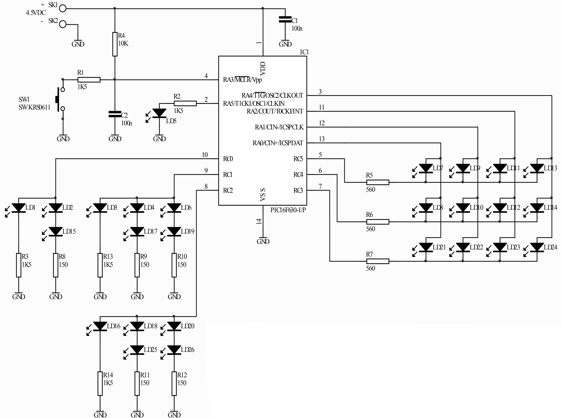
Schematic Diagram MK175
