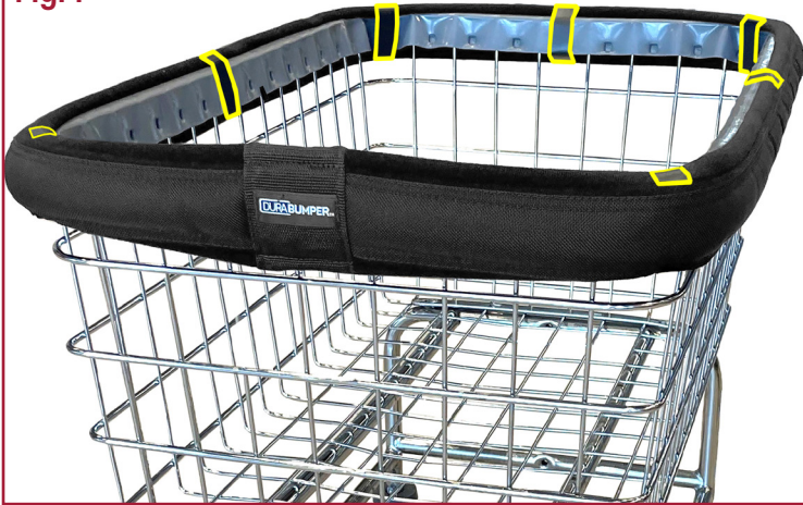
Fig. 1 – Bumper & Velcro® Placement
