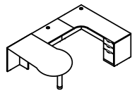
Conference Bullet U-Station with Back Inner Curve PL106/193/182L/166 71"W x 104"D List $1358
