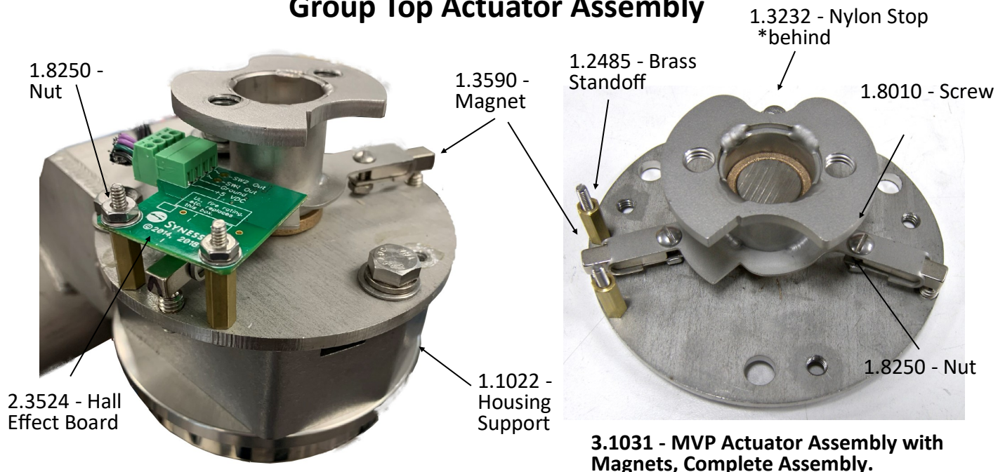
1.1135 - MVP & MVP Hydra Group Top Assembly with Hall Effect Board, Mount Plate, Skirt, Magnets & Hardware
