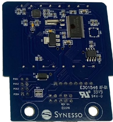
2.3523—Digital Shot Timer Control Board with LED Digits, (Housing and Cover Not Included)
