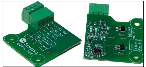
2.3607- Solenoid Switch with Removable Terminal Connector *For Machines After Serial Number xxxxx5683
