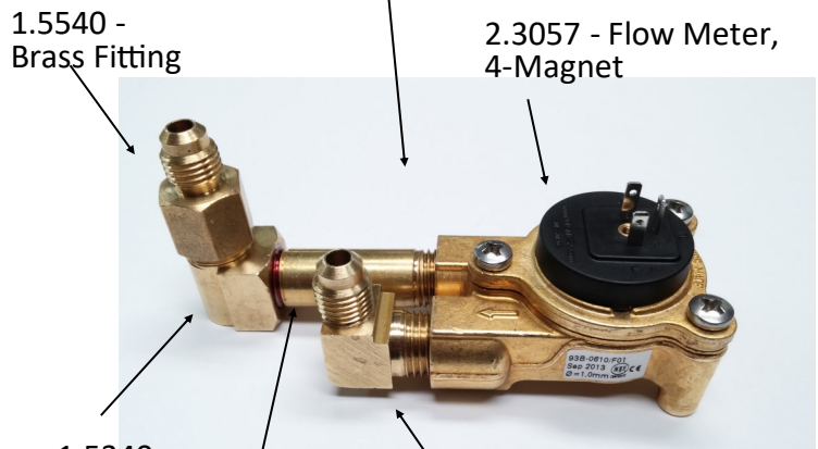
2.3055 - MVP Hydra Flowmeter Assembly (Flowmeters and Brass Fittings. Copper Tubes Not Included in the Assembly.)
