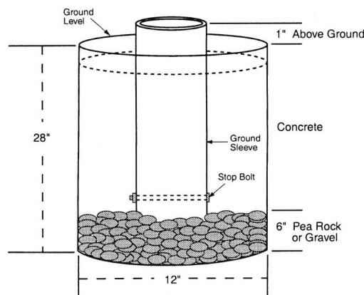
Hole Diagram
