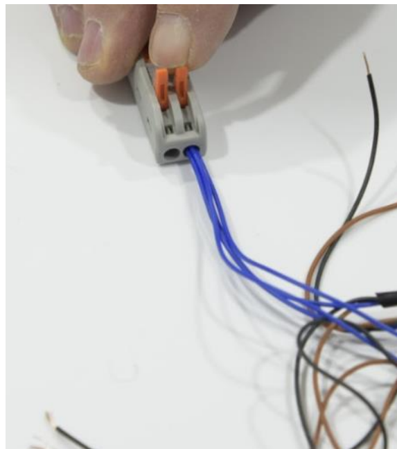
Locking lever open
