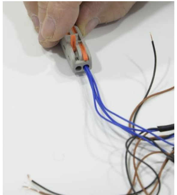
Locking lever closed
