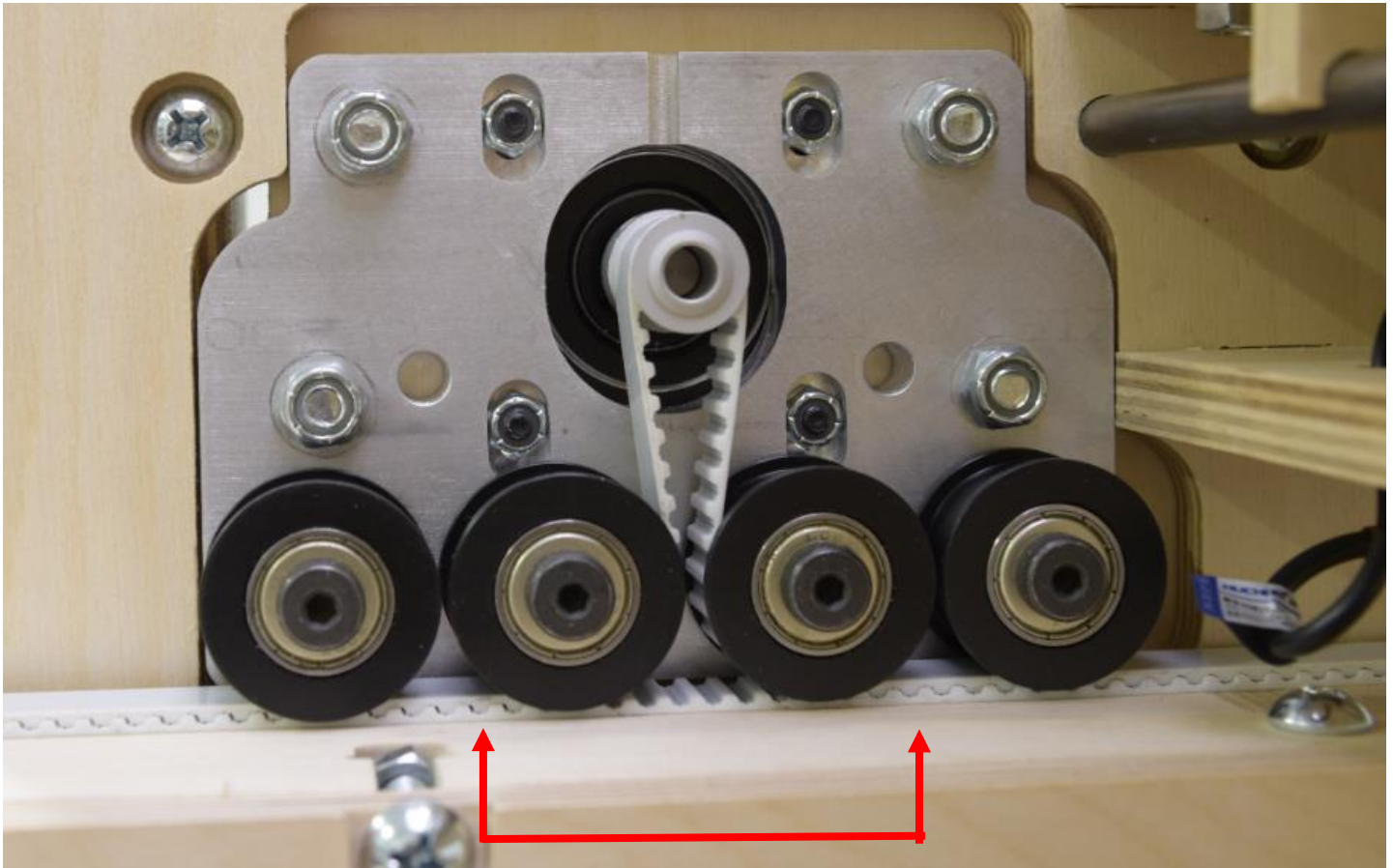
Properly tightened belt with teeth fully engaged beneath the Idler Pulleys.
