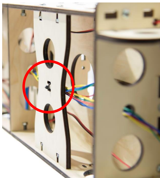
28f Wire Management: Bundle and secure the Stepper Motor Wires to the back of the Gantry Back Support with a Zip Tie as shown.
