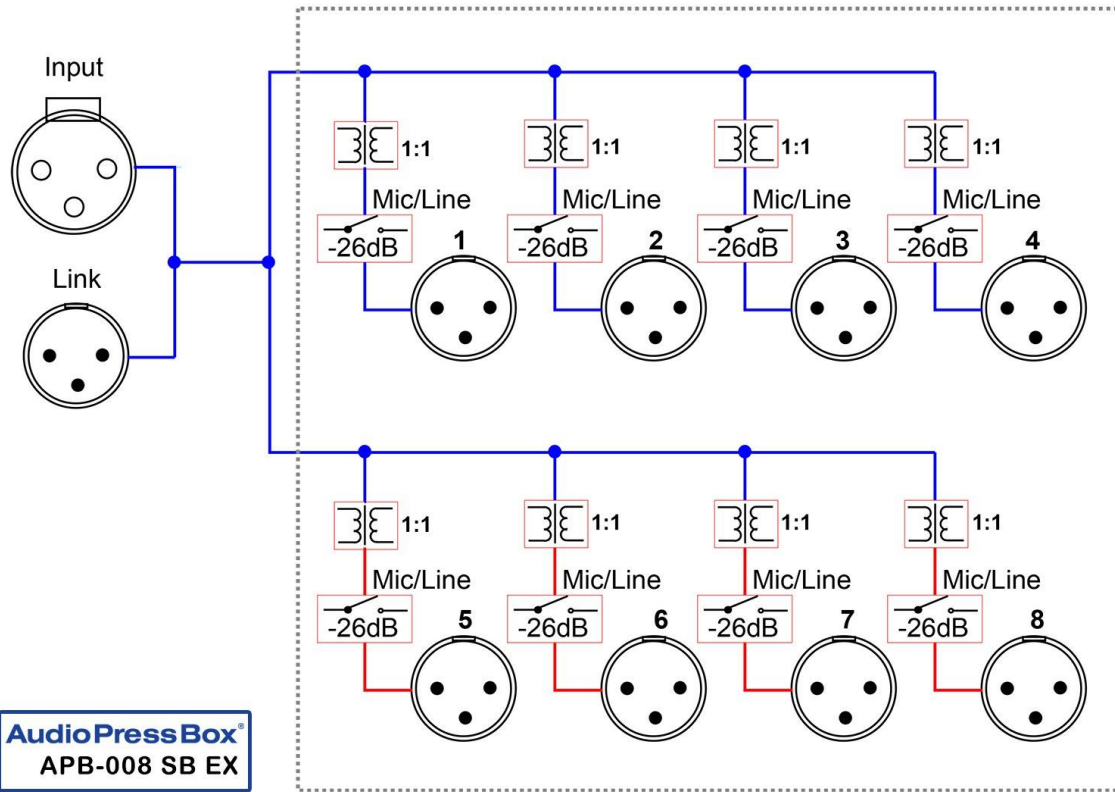
BLOCK DIAGRAM APB-008 SB-EX
