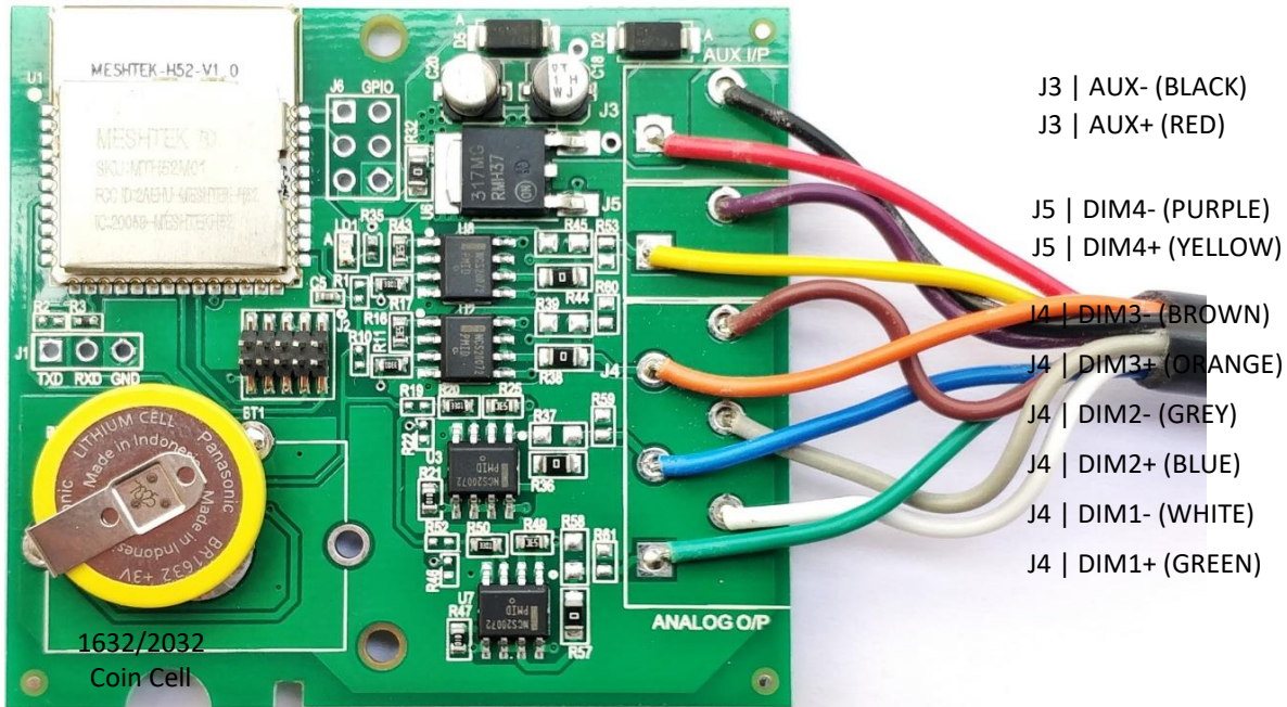
Figure 2-1 B. MeshTek® 4 Channel 0-10V SLC (56mm X 52mm)
