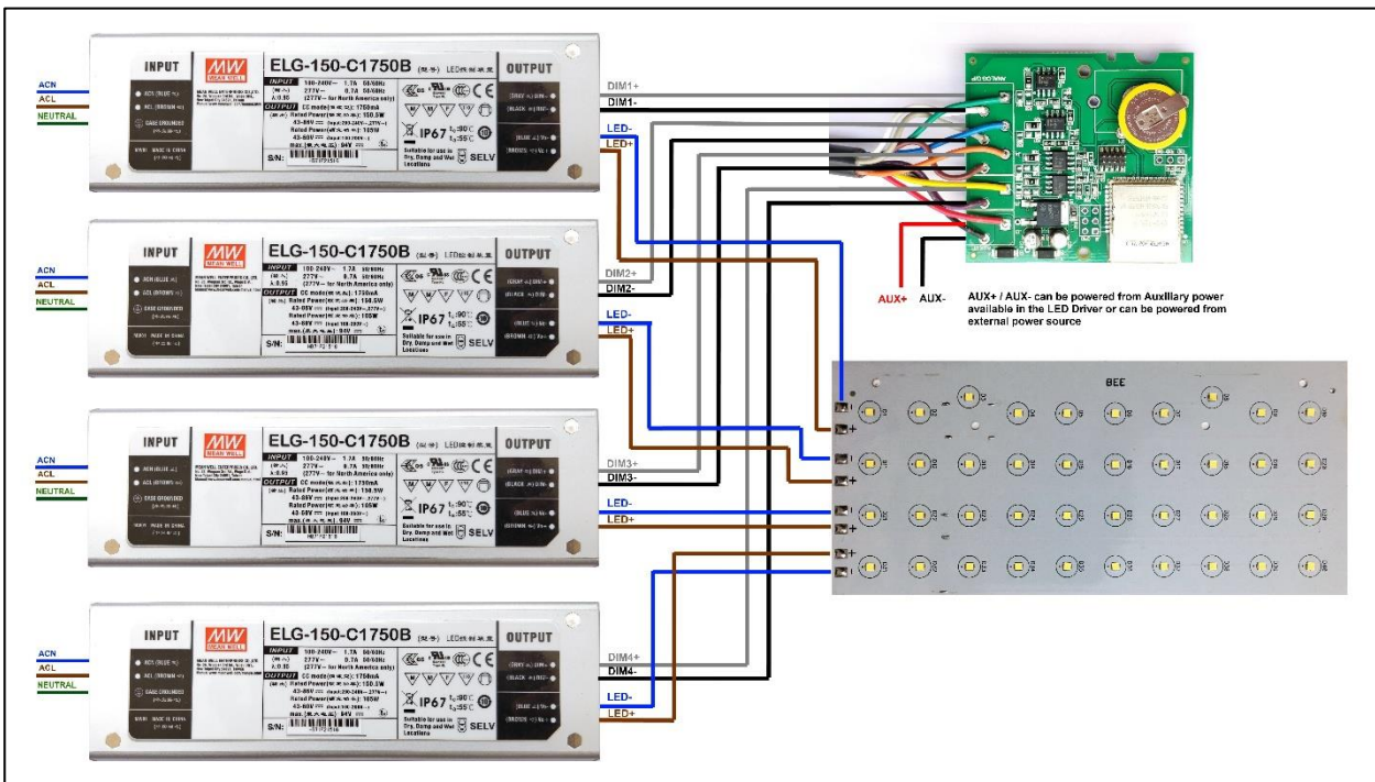
Figure 4-1 Application Setup (Single Channel and Four Channel 0-10V SLC)
