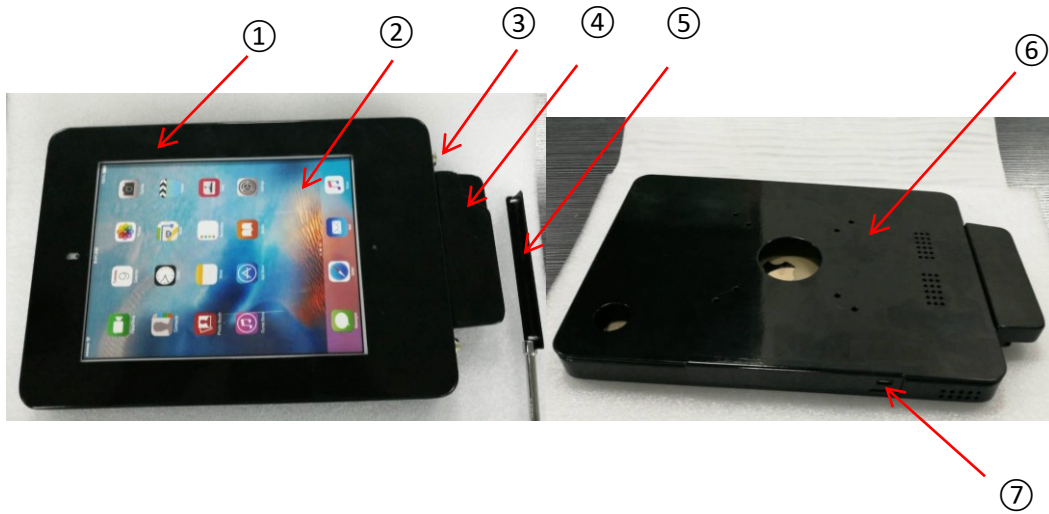
①Front Cover ②iPad ③Lock ④Credit card reader case ⑤Panel ⑥Bottom ⑦Micro usb port
