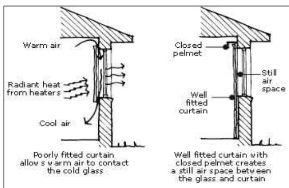
Heat loss with and without pelmets
