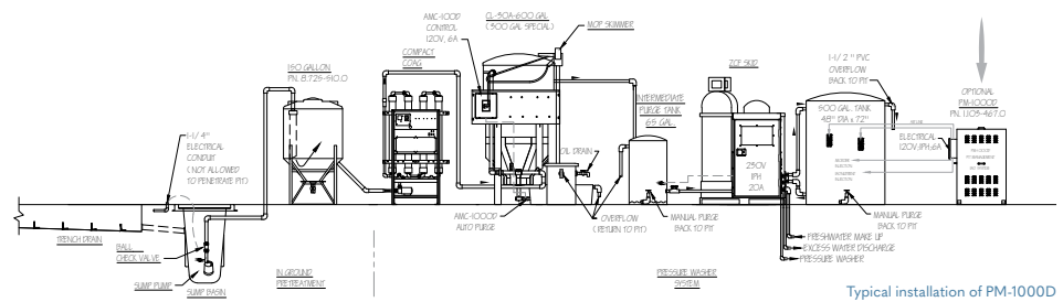
Typical installation of PM-1000D
