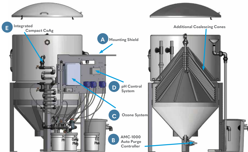
01 Universal Clarifier System with Coalescing Cones and Funnel Skimmer
