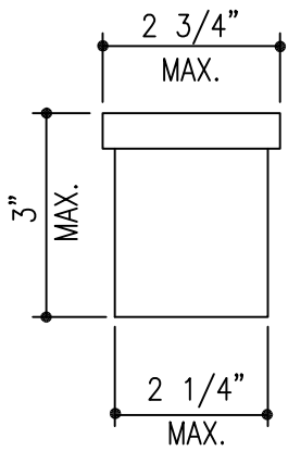
SPECIMEN CUP MAXIMUM DIMENSIONS
