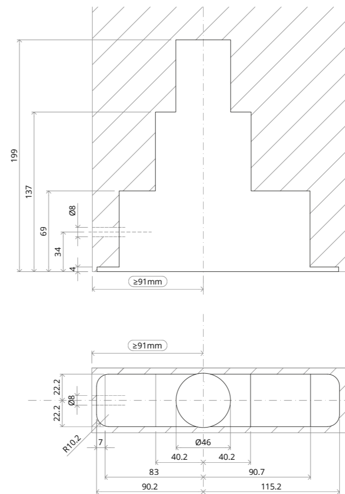
MILLING DRAWING
