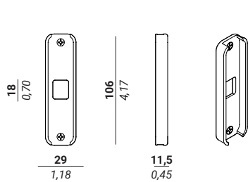
Dimensioni contropiastra / Counterplate dimensions
