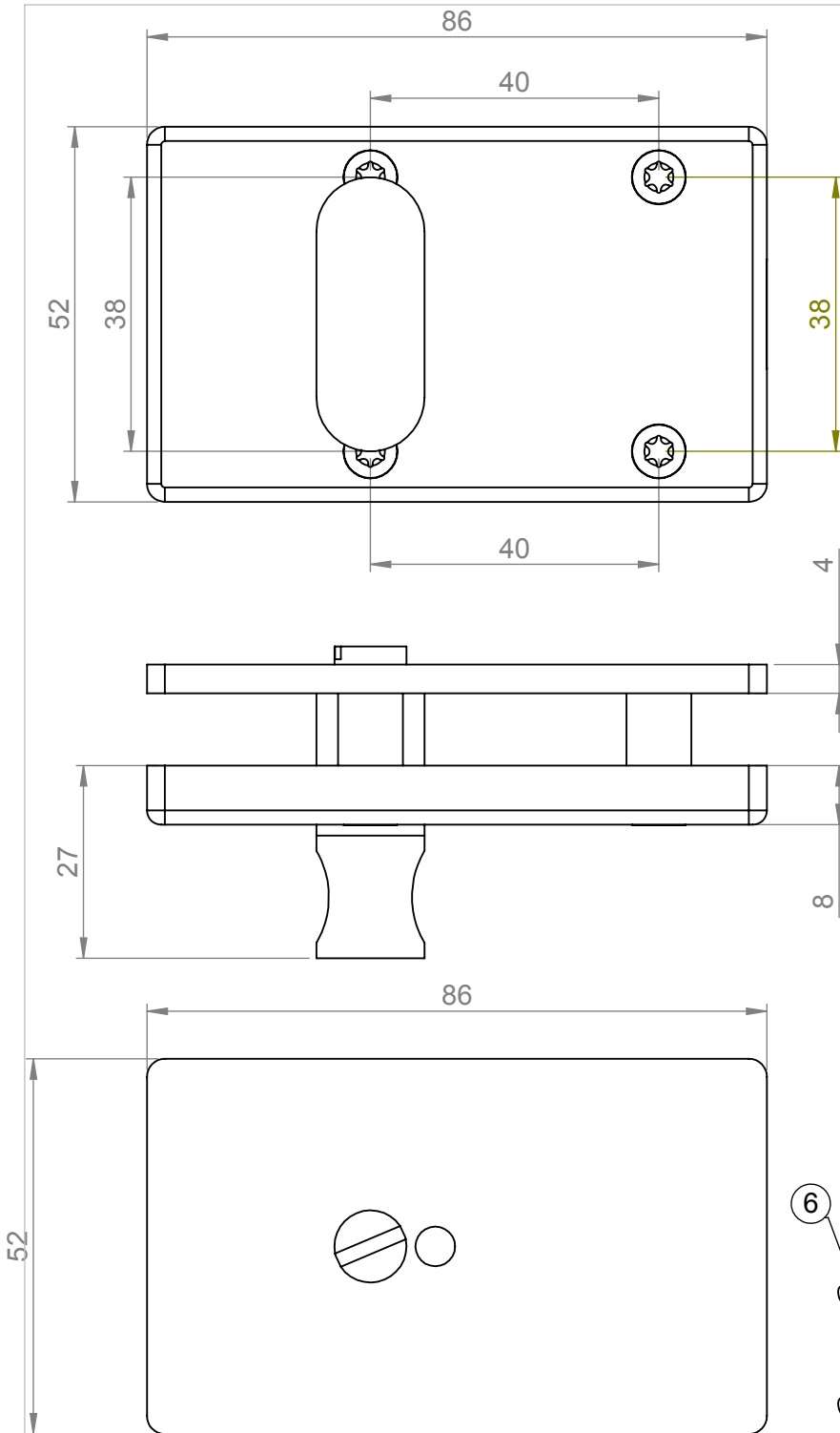
14.9736.02.013 Strike plate 90angel 14.9736.02.021 Strike plate for surface
