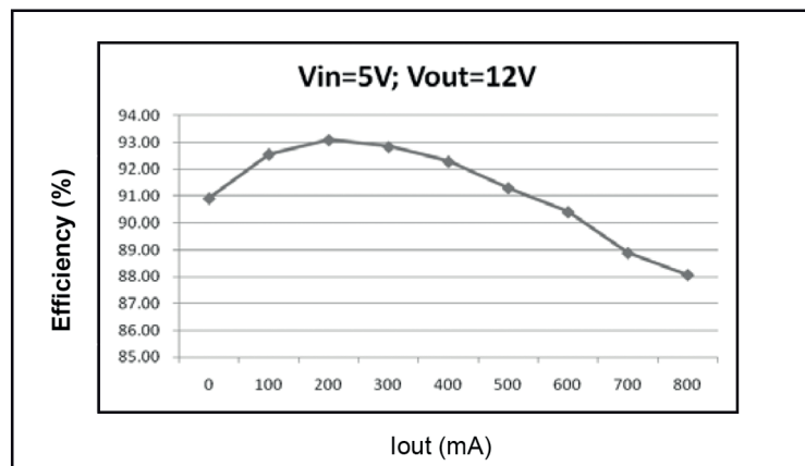
Figure 2. Efficiency Curve
