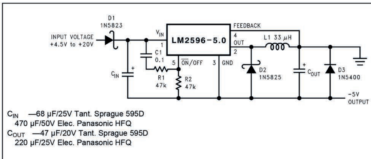
Figure 37. Inverting -5V Regulator with Delayed Startup
