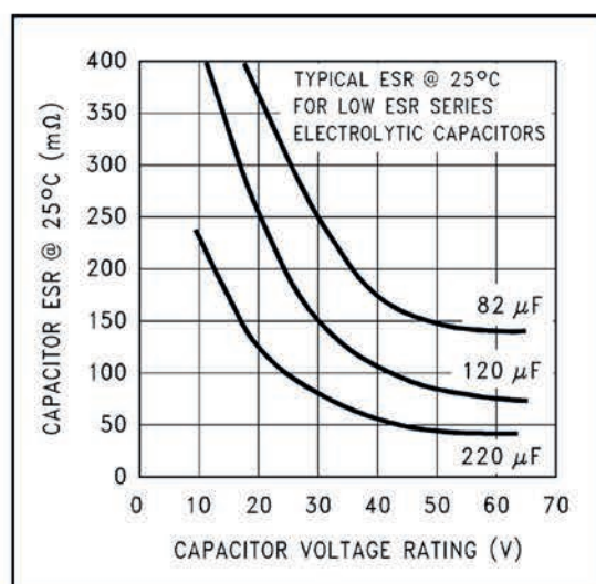
Figure 26. Capacitor ESR vs Capacitor Voltage Rating (Typical Low ESR Electrolytic Capacitor)
