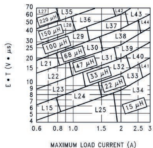
Figure 24. LM2596-ADJ
