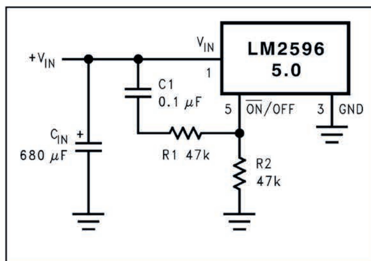
Figure 33. Delayed Startup
