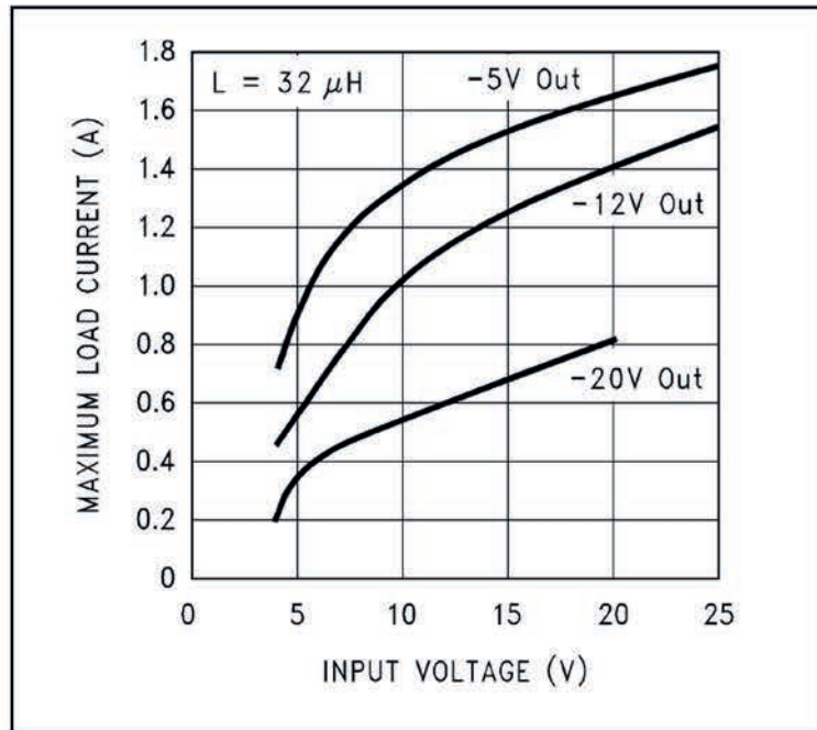
Figure 38. Inverting Regulator Typical Load Current
