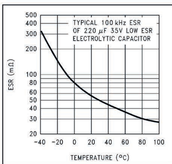
Figure 27. Capacitor ESR Change vs Temperature
