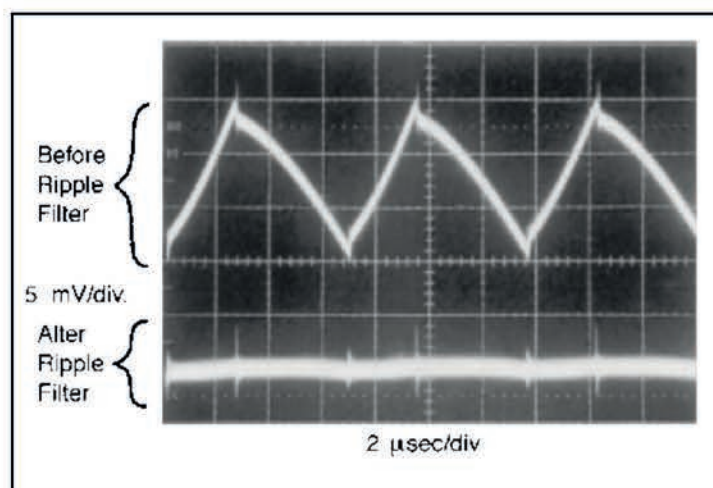
Figure 29. Post Ripple Filter Waveform
