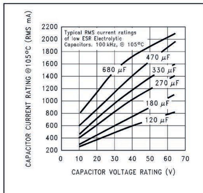
Figure 25. RMS Current Ratings for Low ESR Electrolytic Capacitors (Typical)
