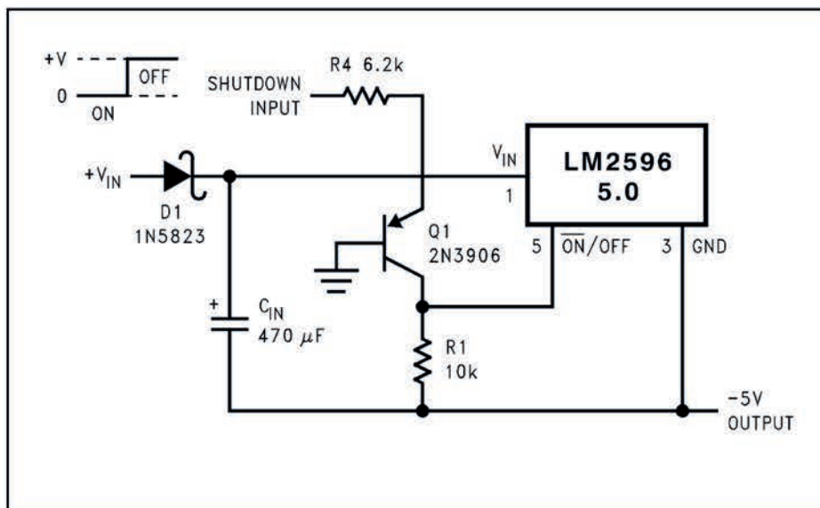
Figure 39. Inverting Regulator Ground Referenced Shutdown
