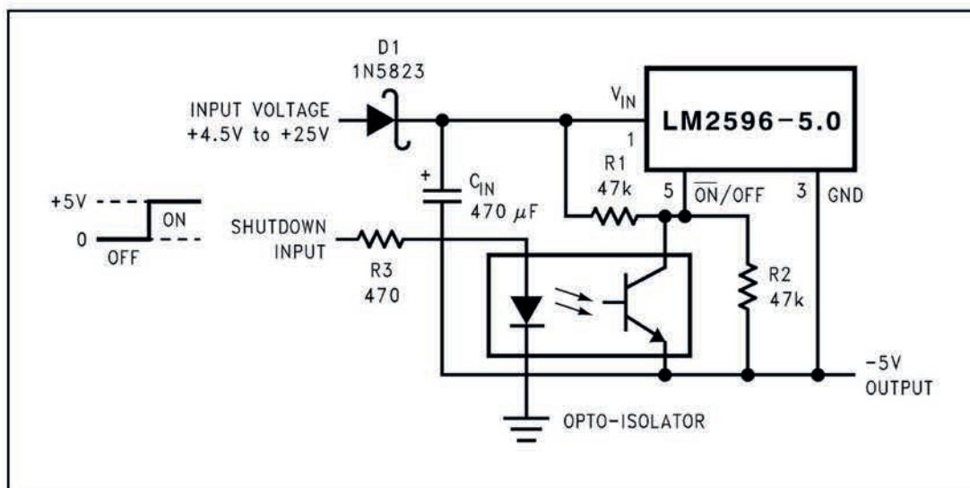
Figure 40. Inverting Regulator Ground Referenced Shutdown using Opto Device
