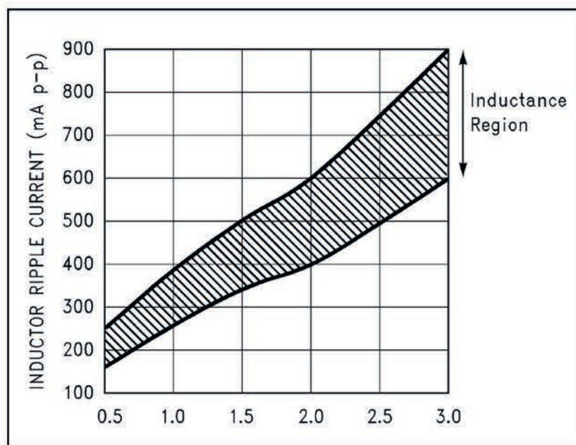
Figure 30. Peak-to-Peak Inductor Ripple Current vs Load Current
