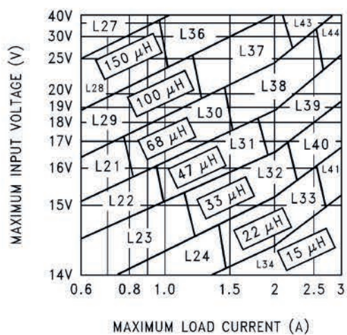
Figure 23. LM2596-12
