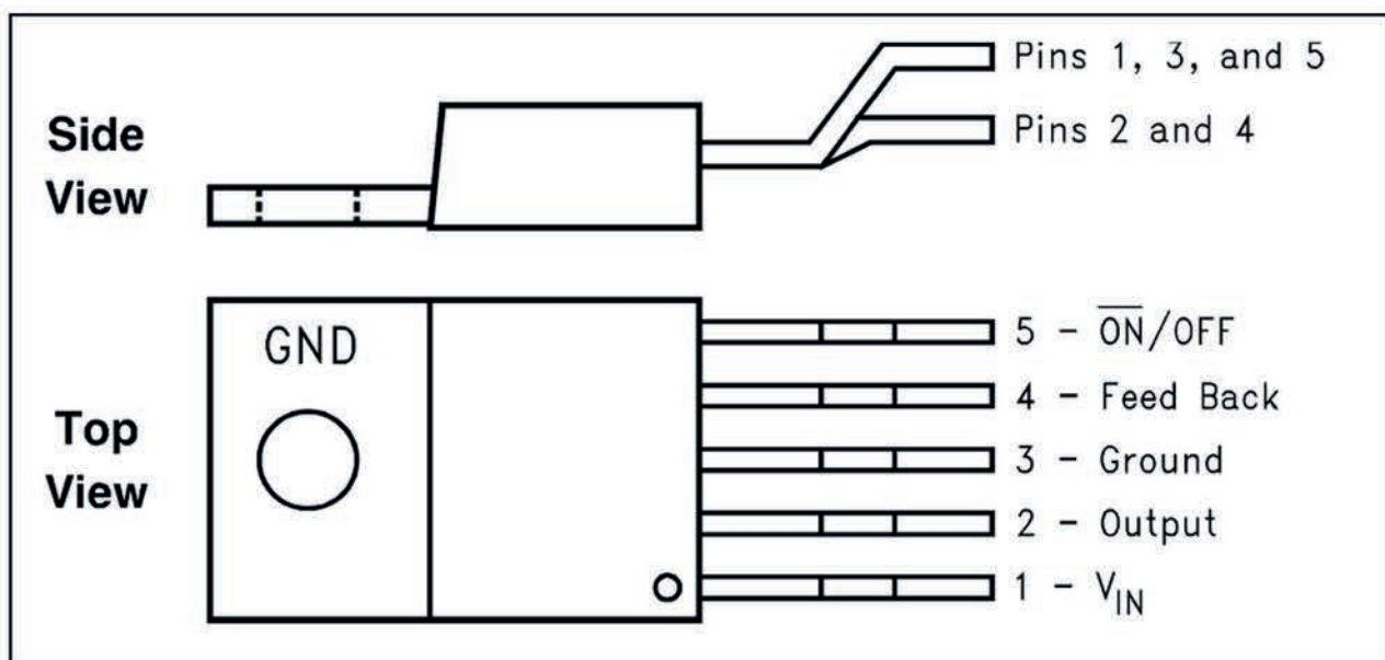
Figure 1. 5-Lead Bent and Staggered Leads, Through Hole TO-220 (T) Package
