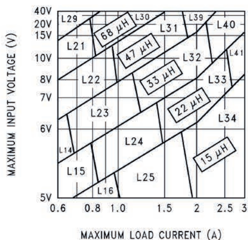
Figure 21. LM2596-3.3
