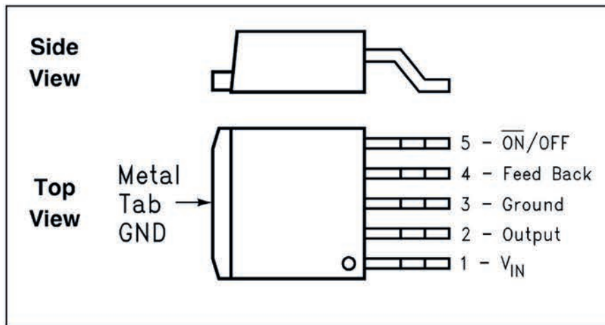
Figure 2. 5-Lead DDPAK/TO-263 (S) Package
