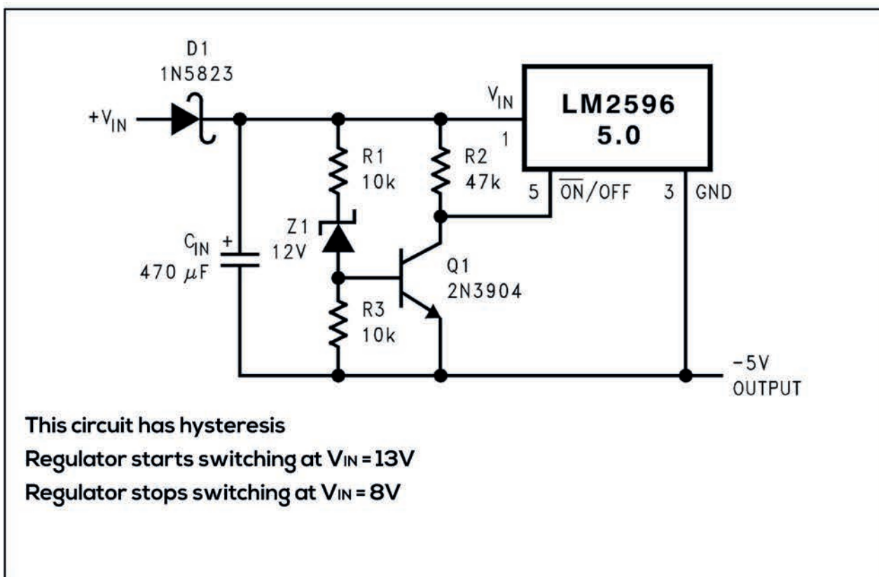
Figure 36. Undervoltage Lockout with Hysteresis for Inverting Regulator
