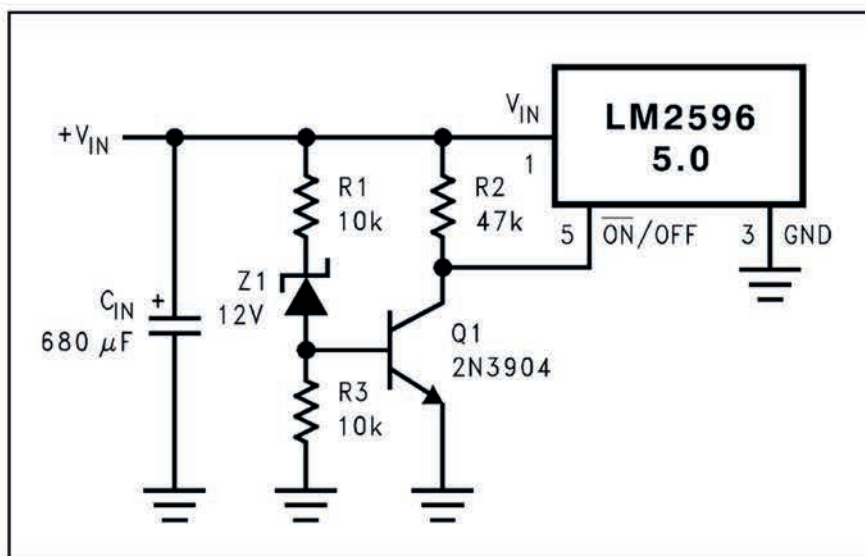
Figure 34. Undervoltage Lockout for Buck Regulator
