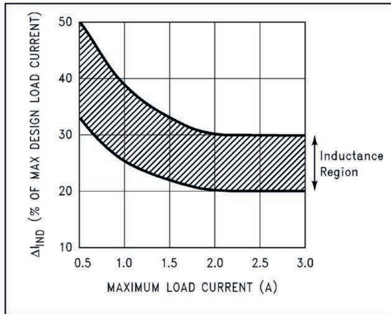
Figure 28. ( \Delta I_{IND} ) Peak-to-Peak Inductor Ripple Current (as a Percentage of the Load Current) vs Load Current
