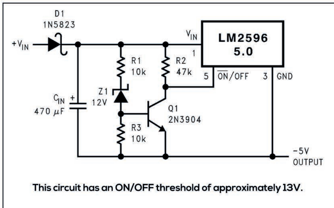
Figure 35. Undervoltage Lockout for Inverting Regulator
