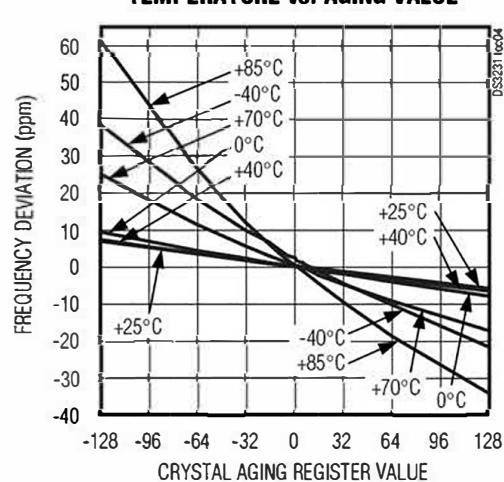
FREQUENCY DEVIATION vs. TEMPERATURE vs. AGING VALUE
