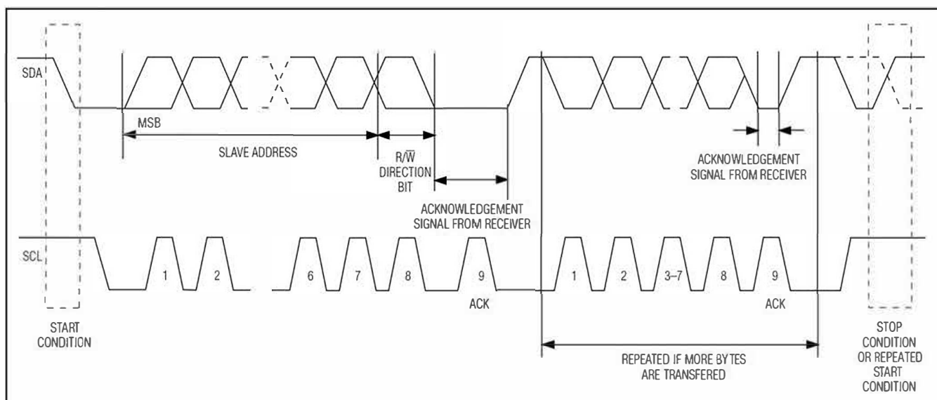
Figure 2. I²C Data Transfer Overview
