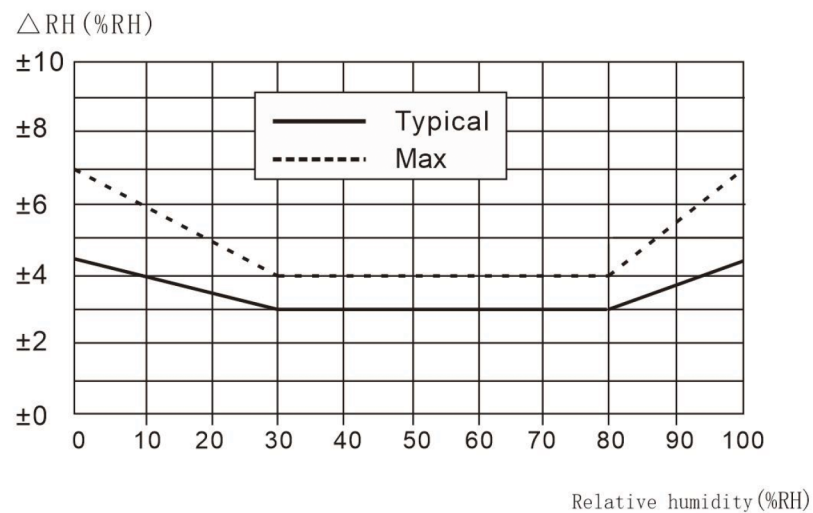
Figure 2. Typical and maximum humidity errors
