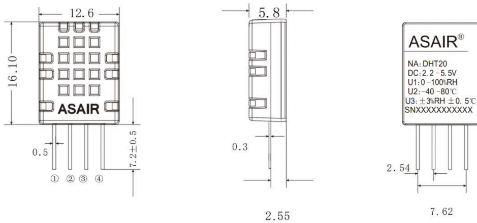
Figure 13. DHT20 sensor encapsulation (unit: mm not specified tolerance: \pm 0.2 mm)
