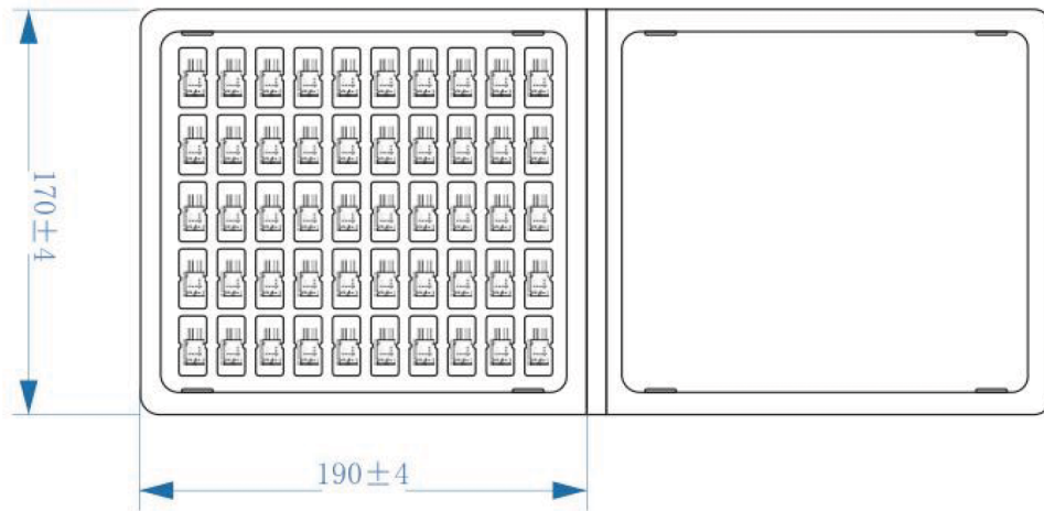
Figure 12. DHT20 sensor package diagram (unit: mm unmarked tolerance: \pm 0.2 mm)
