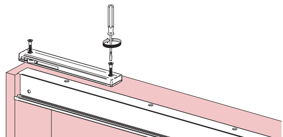
Travão porta central
