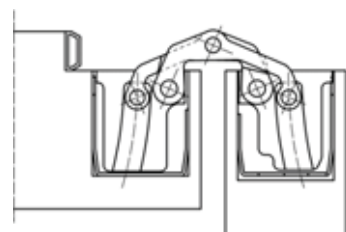
Blockzarge 180°
