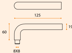
BZ.00.028.RC08M TIMES Material: Bronze / Bronze / Bronze Puxador com roseta / Lever handle with rose / Manillas con roseta.
