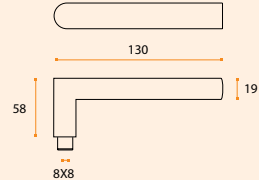
BZ.00.030.RC08M TIMES Material: Bronze / Bronze / Bronze Puxador com roseta / Lever handle with rose / Manillas con roseta.
