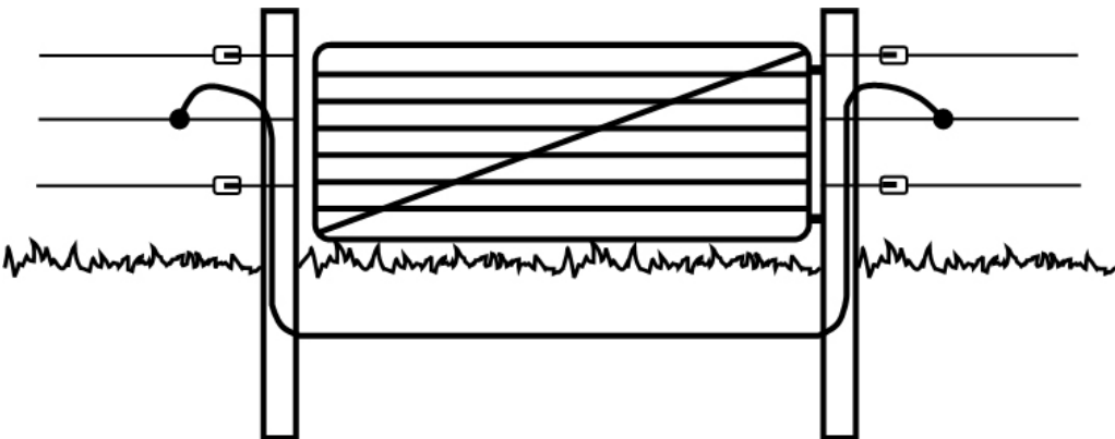
Steel Gate example
