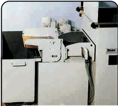
Magnetic separator for cleaning of coolant water
