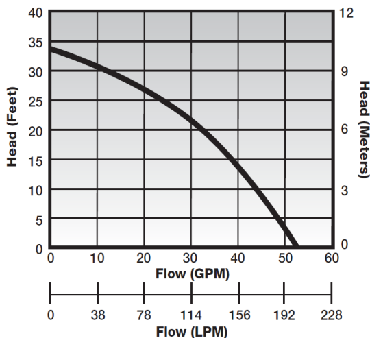
Model CCT-457-15
