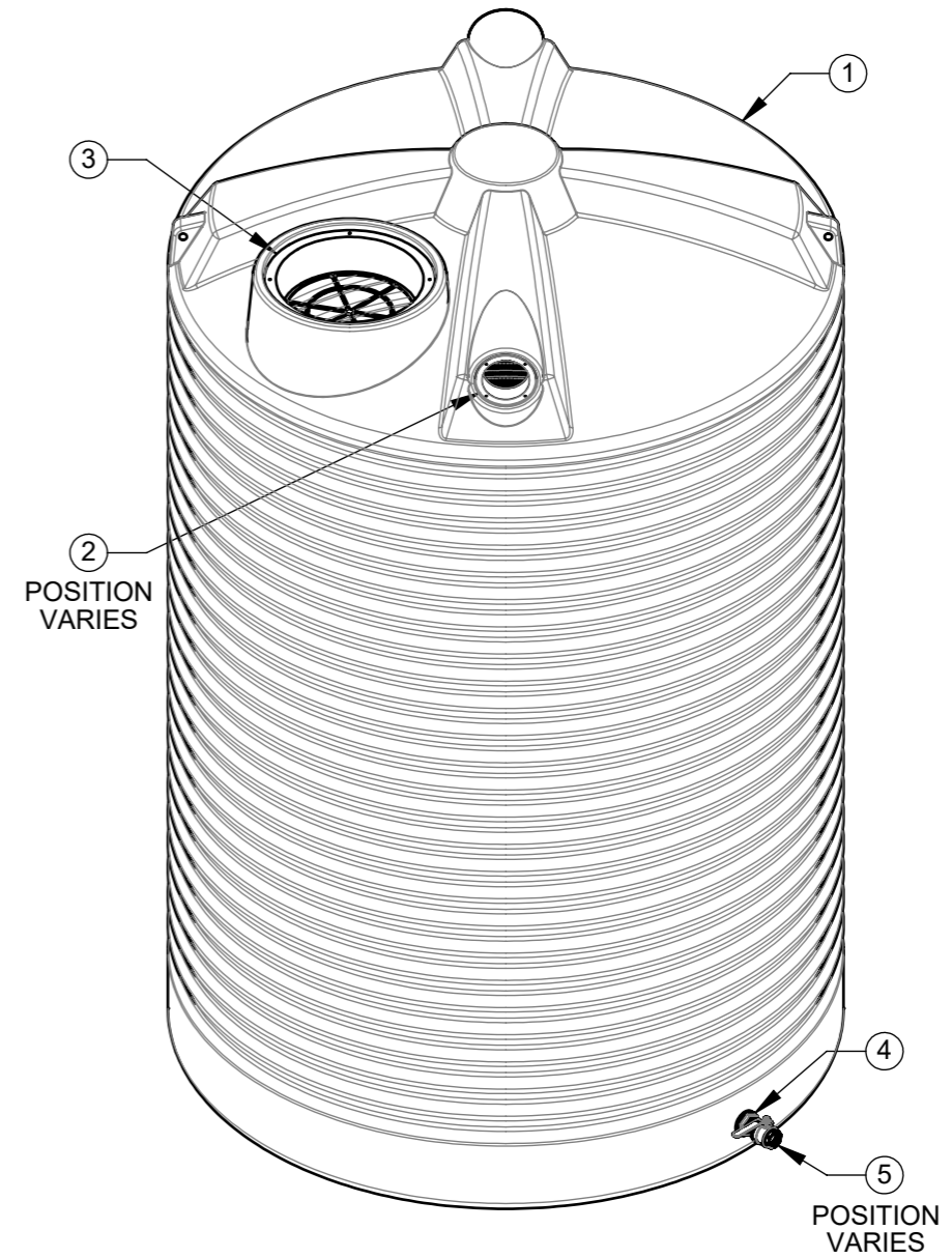
ISOMETRIC VIEW
