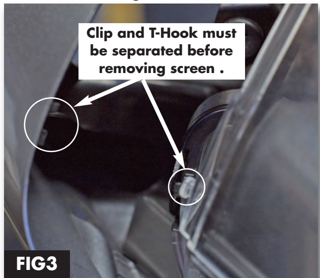
Fig 3. Separate T-Hooks from the retention clip by applying a light pressure from the corner fairing and work the light pressure down as shown. (Both Sides) Be careful not too exert to much force!
