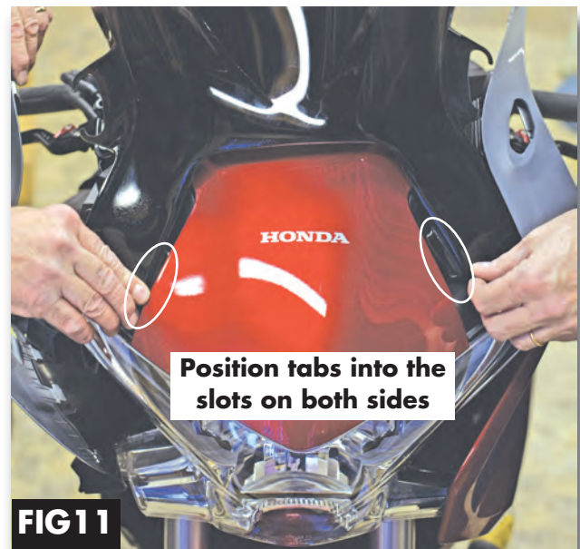
FIG 11 Fig 11. Carefully pull back on the top side fairing while slipping the ZG screen tabs into the appropriate slots. Use the mirror mounting point for a reference to position the screen. Install provided allen screws and plastic washers. Bolt on side mirrors to finish.
