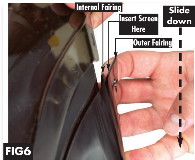
Fig 6. HERE IS THE TRICKY PART! Now you are ready to insert the corner screen into the fairing. At the corner of the fairing, apply light pressure to lift and expose the hidden internal fairing. Looking from the top of the fairing, in front of the windscreen. Insert the corner of the windscreen plastic to the top of the internal fairing. As shown above. Apply light pressure separating the internal fairing and the outer fairing. This separation will provide the screen to slide into the fairing. Once both corners are positioned, slide the screen down using equal pressure.
