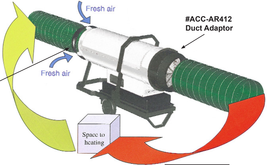
#ACC-AR412 Duct Adaptor
